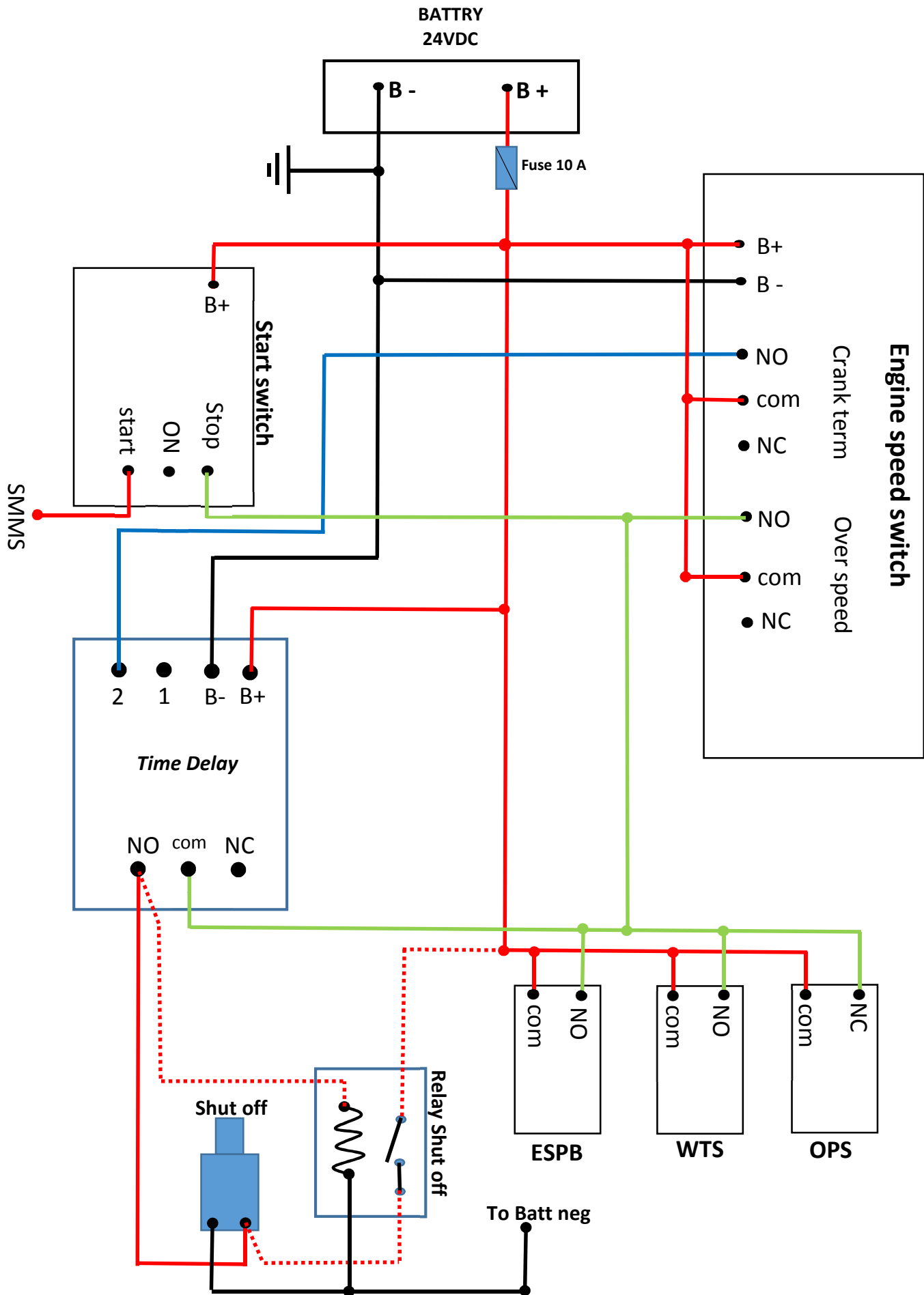
Wiring D3306 for start stop with time delay and ESS
